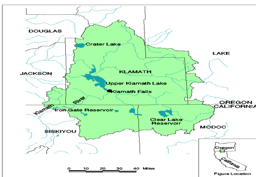
Figure 1. --Upper Klamath Basin ground-water study area.
